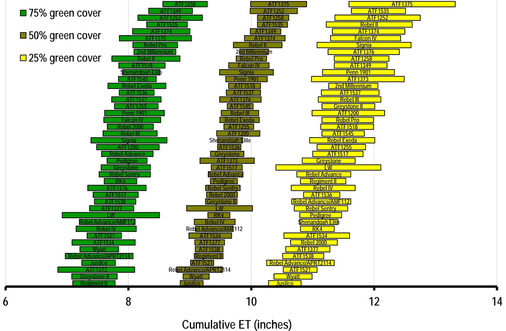
Figure 4. Confidence intervals (95%) for the amount of moisture lost to evapotranspiration after irrigation is withheld before selections from data set 09AFA1 reach 75, 50, and 25% green cover.
