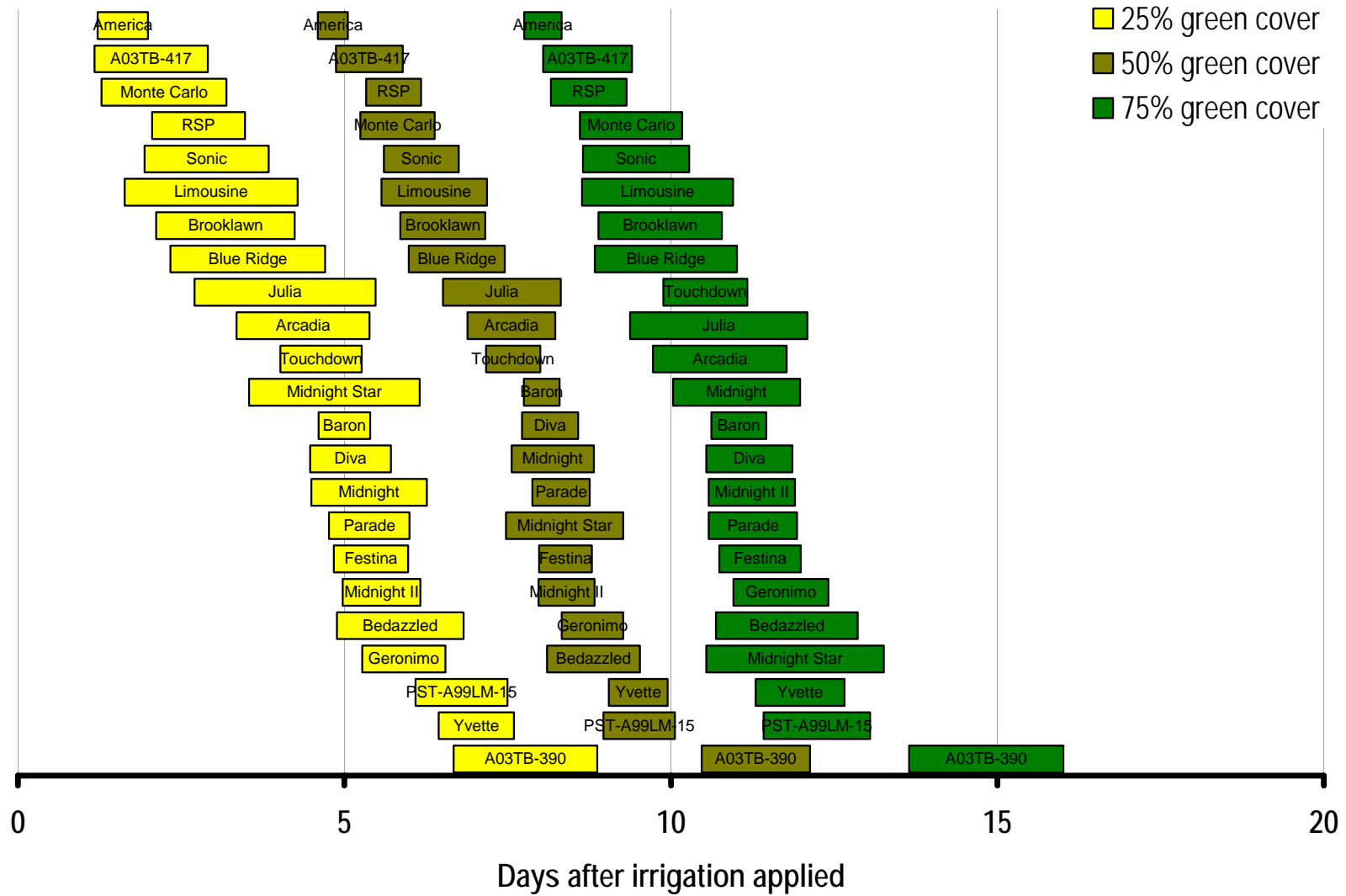
Figure 6. Confidence intervals (95%) for the number of days after irrigation is applied before varieties reach 25, 50, and 75% green cover in 2006.
