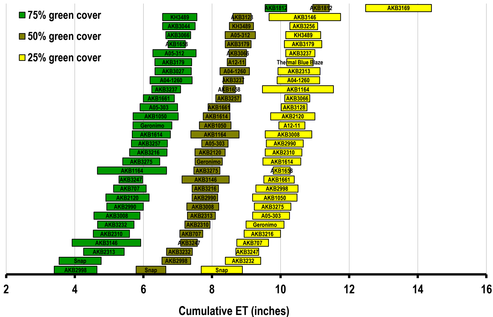
Figure 4. Confidence intervals (95%) for the moisture lost to evapotranspiration before the bottom-performing (bottom half) of 58 Kentucky bluegrass entries from data set 13APP1 reach 75, 50, and 25% green cover. Both the top and bottom performing entries are included for reference.
