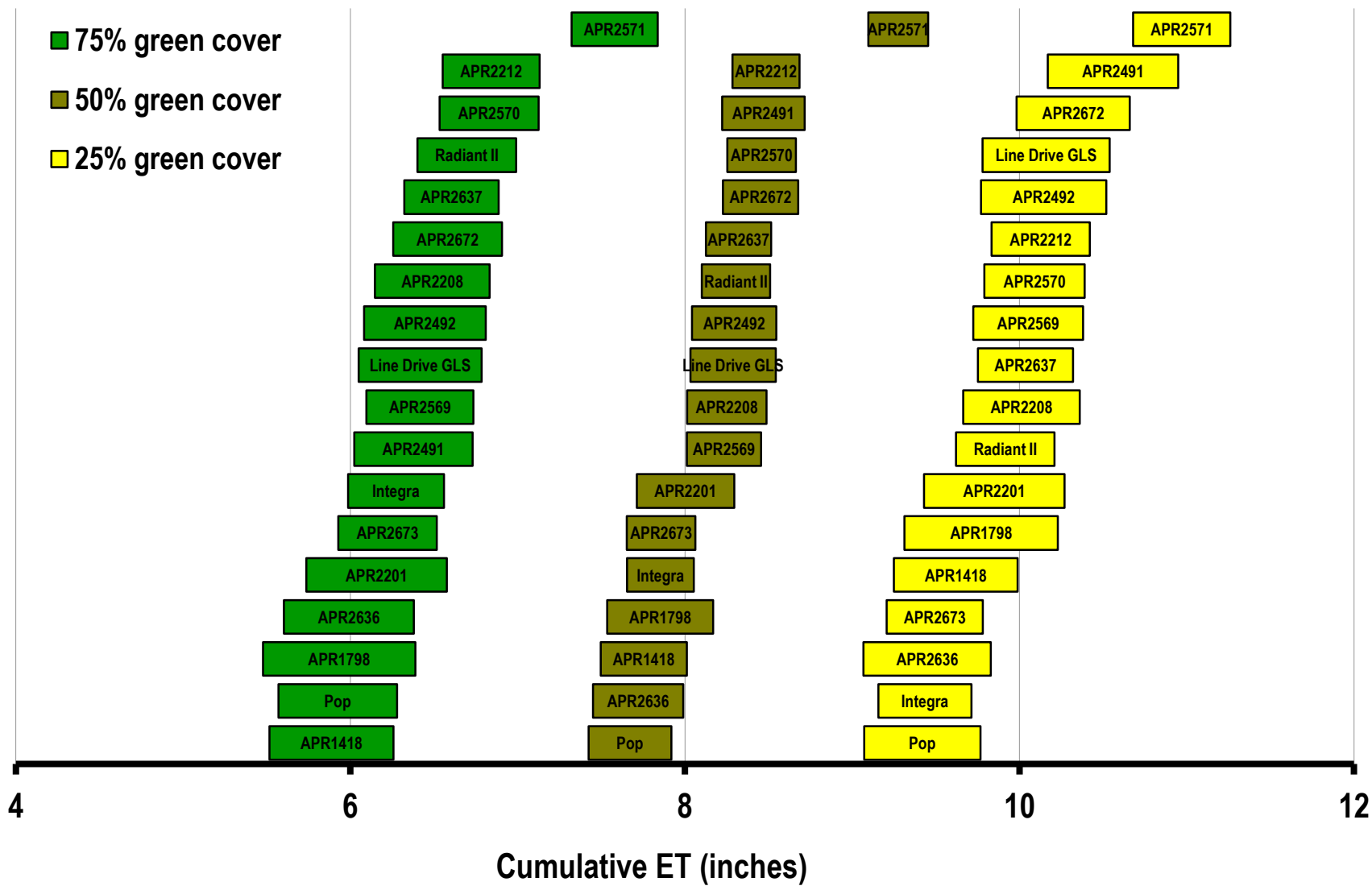
Figure 2. Confidence intervals (95%) for the moisture lost to evapotranspiration before the 18 perennial ryegrass entries from data set 12ALP2 reach 75, 50, and 25% green cover.
