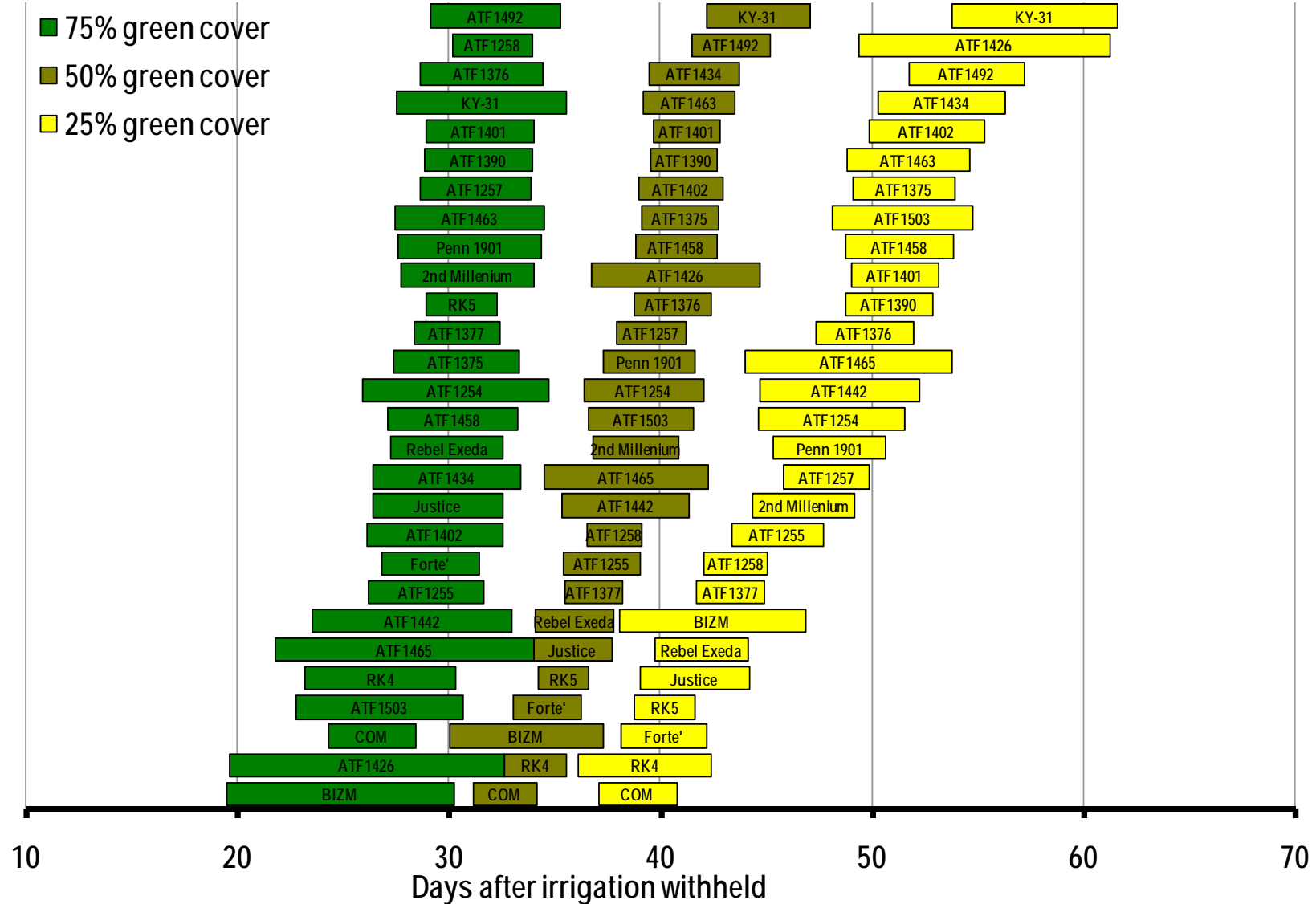
Figure 4. Confidence intervals (95%) for the number of days after irrigation is withheld before selections reach 75, 50, and 25% green cover. Twenty-eight of 125 selections are shown here to represent the range of drought tolerance present in this data set. Confidence intervals for all 125 selections are listed in Table 2.
