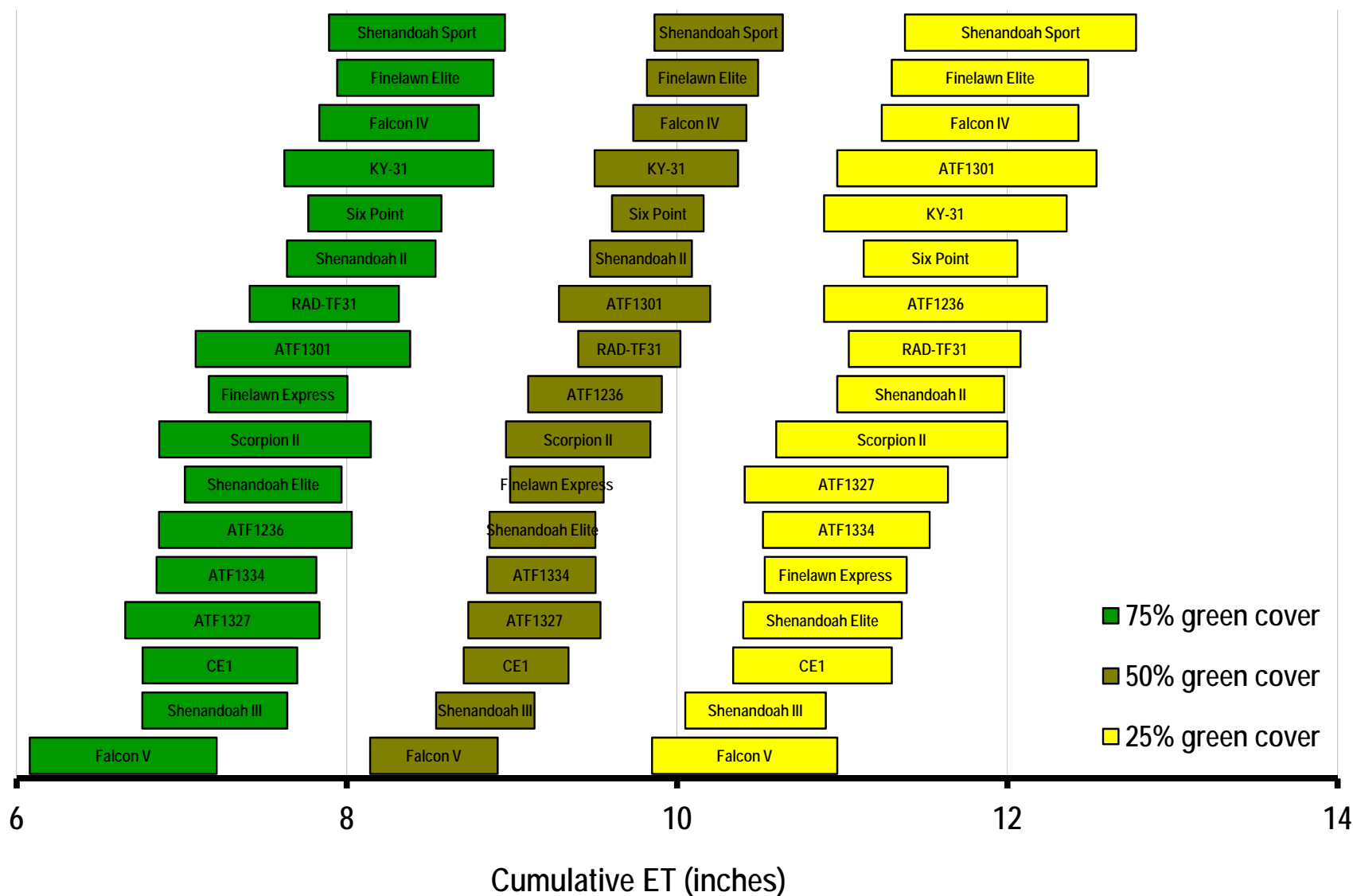
Figure 4. Confidence intervals (95%) for the amount of moisture lost to evapotranspiration after irrigation is withheld before selections from data set 09AFA2 reach 75, 50, and 25% green cover.
