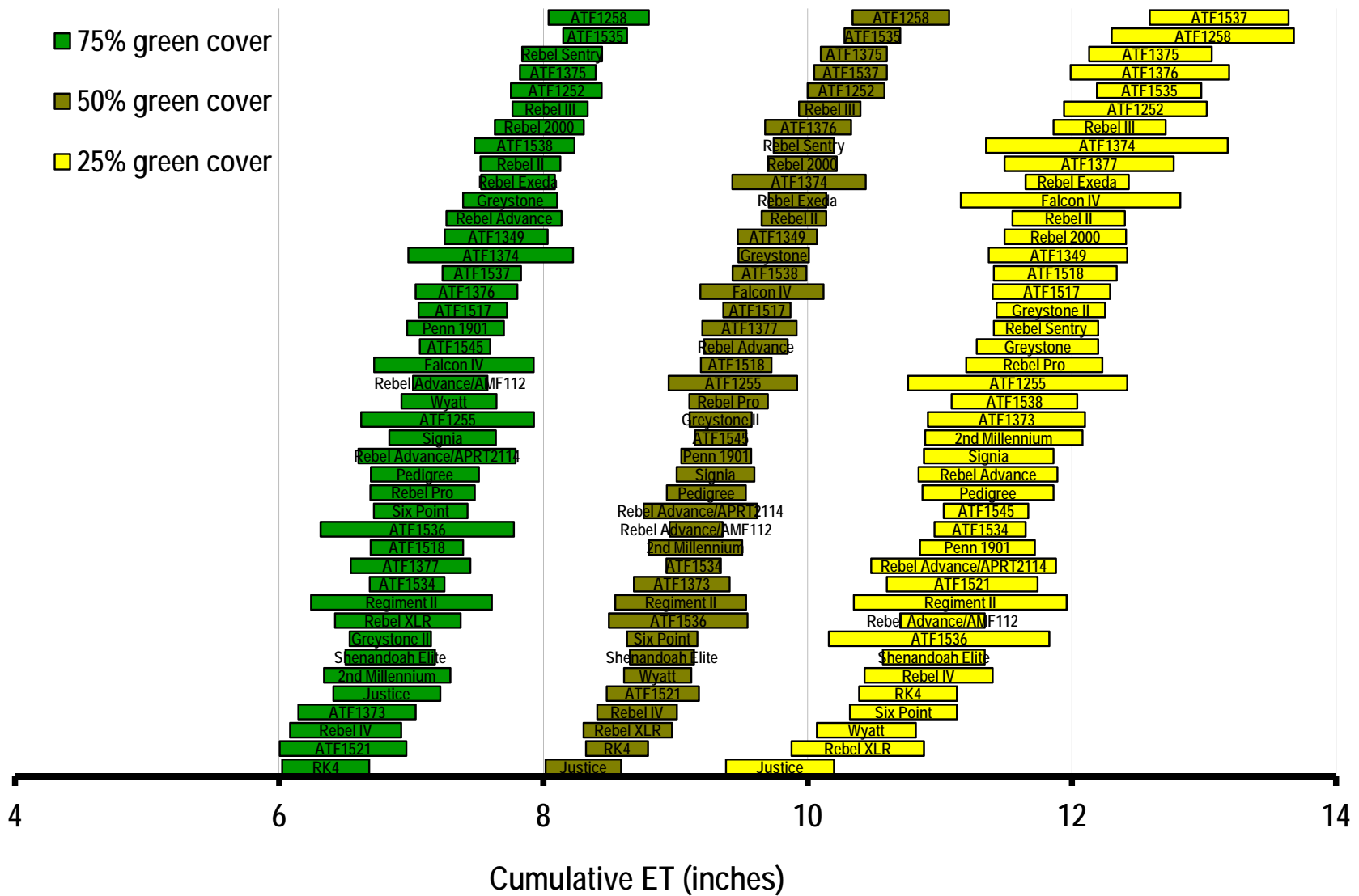
Figure 2. Confidence intervals (95%) for the amount of moisture lost to evapotranspiration after irrigation is withheld before selections (09AFA1 data set) reach 75, 50, and 25% green cover. 75 and 50% cover is from actual data, 25% is extrapolated.
